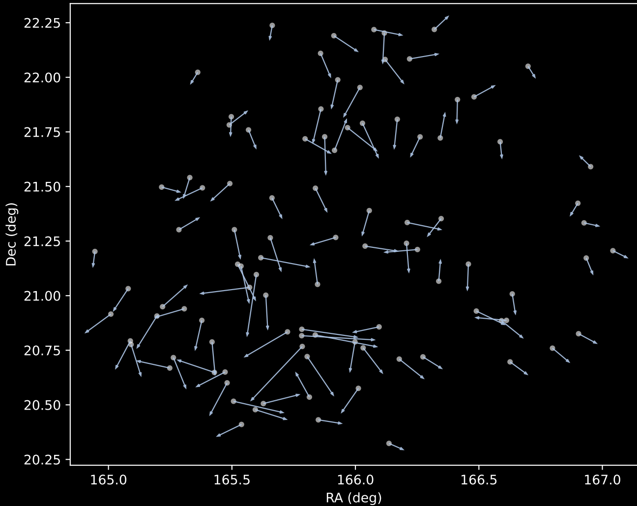
GALAH DR4 Cluster 1 Proper Motion Vectors (n=98)
