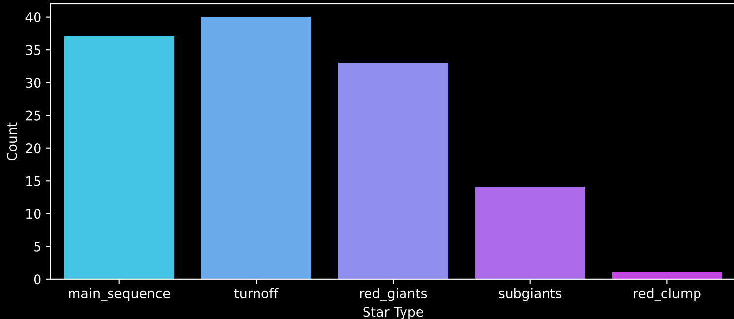
GALAH DR4 Field: [6792] Count plot of Star Type
