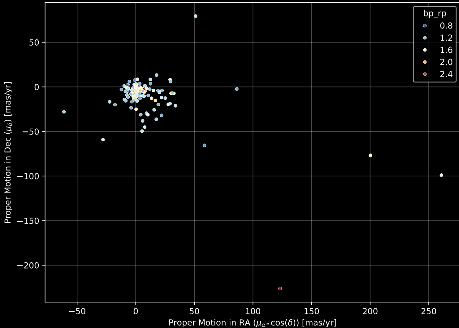
GALAH DR4 Field: [6792] Proper Motion Diagram (n= 125)
