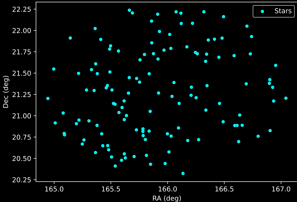
GALAH DR4 Field: [6792] Proper Motion Vectors for Gaia Star Field (n= 125)
