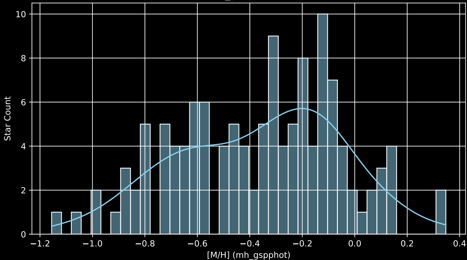
GALAH DR4 Field: [6792] [M/H] (mh_gspphot) (n= 125)
