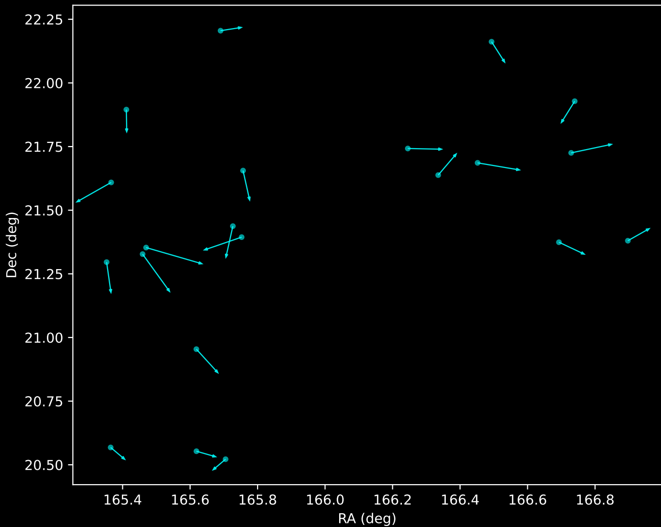
GALAH DR4 Noise Stream Proper Motion Vectors (n=21)
