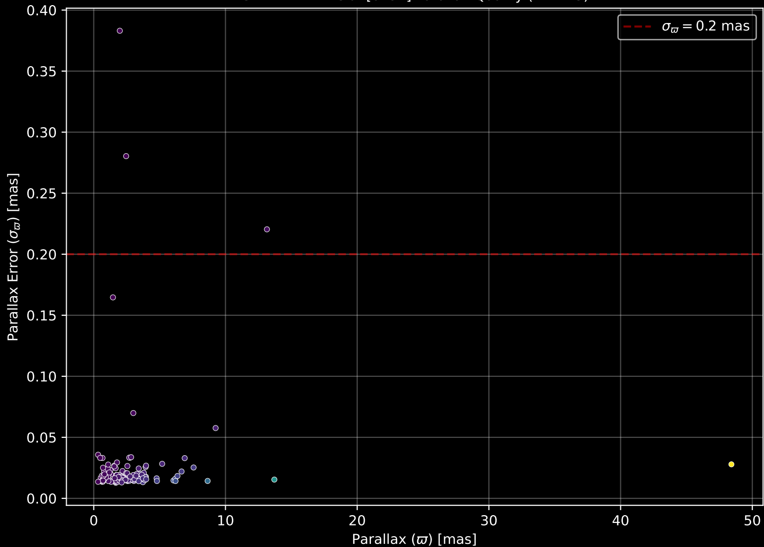
GALAH DR4 Field: [6792] Parallax Quality (n= 125)
