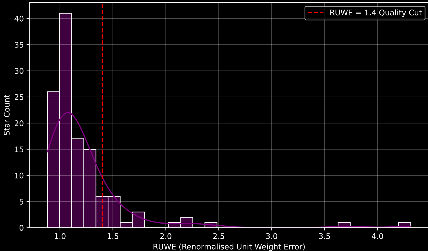
GALAH DR4 Field [6792] RUWE Distribution (n= 121)
